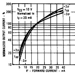
Normalized Output Current vs Input Current
