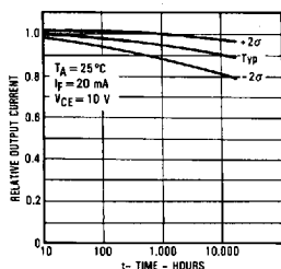
Relative Output Current vs Time
