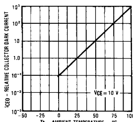
Collector Dark Current vs Ambient Temperature
