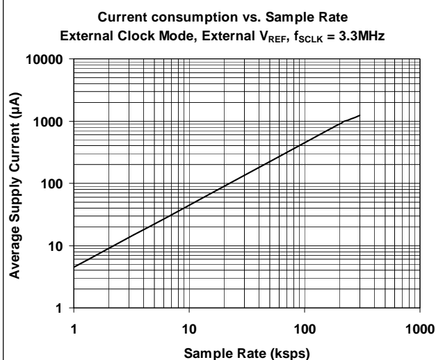
Figure 18: Supply Current versus Sampling Rate
