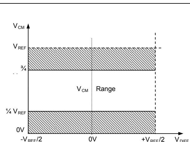
Figure 7: Input voltage range for bipolar mode
