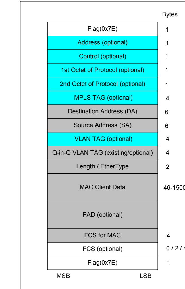
Figure 8-21. HDCL Encapsulated Frame Format
