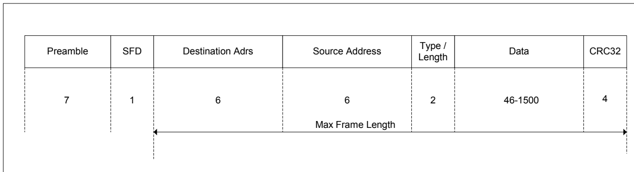
Figure 8-8. IEEE 802.3 Ethernet Frame
