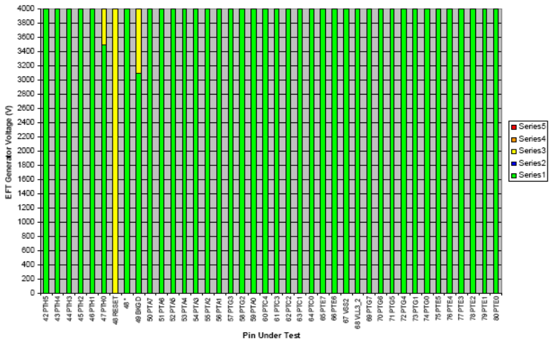
Figure 30. 4 MHz, Negative Polarity Pins 42 – 80
