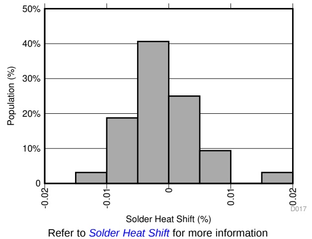
Figure 18. Solder Heat Shift Distribution
