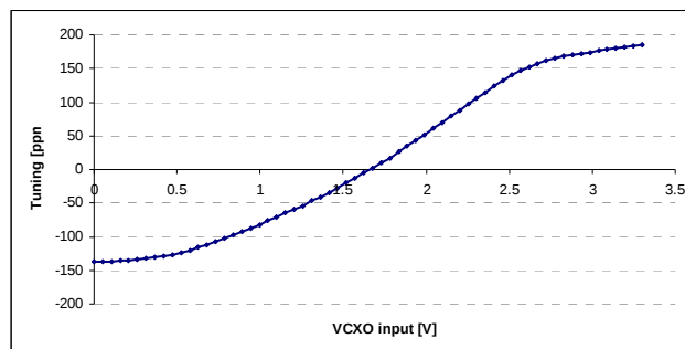
Figure 4. VCXO Profile
