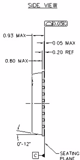
Figure 11. 32-Pin Punch QFN (5 x 5 mm) LY32
