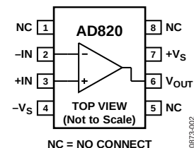
Figure 2. 8-Lead SOIC_N and 8-Lead MSOP
