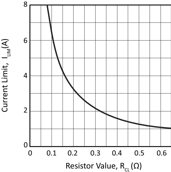
Figure 13: Current Limit
