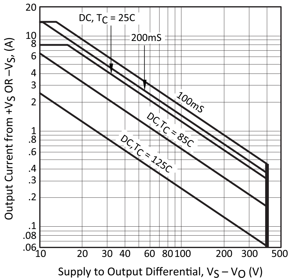
Figure 14: SOA
