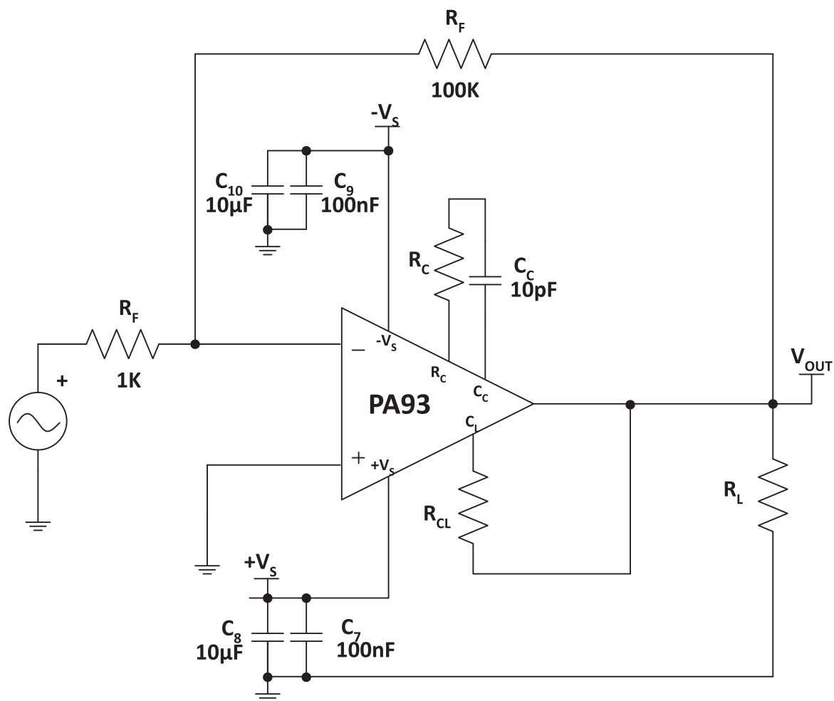
Figure 2: Typical Connections
