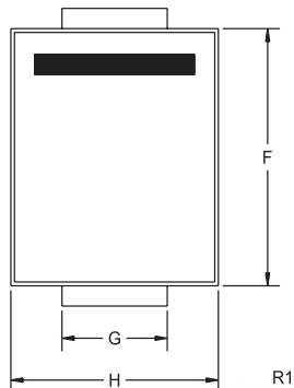
SMC - CASE - MECHANICAL OUTLINE
