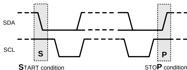
Figure 24. I²C Start Stop Conditions
