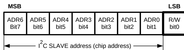
Figure 25. I²C Chip Address
