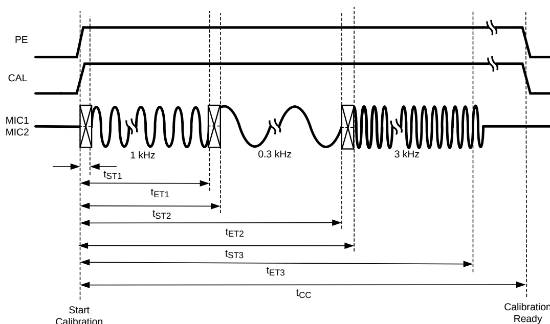
Figure 31. Calibration Timing
