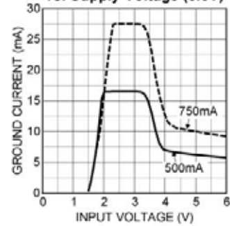
Ground Current vs. Supply Voltage (3.3V)
