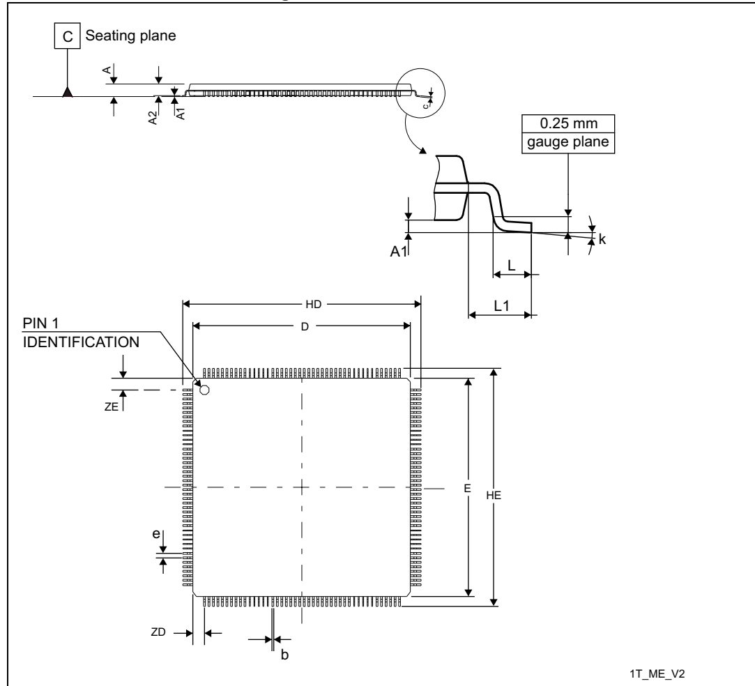
Figure 88. LQFP176 outline
