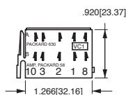
MARKING DETAIL FRONT VIEW
