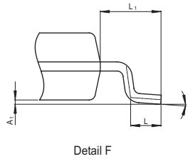
Terminal cross section ( Ni/Pd/Au plating )
