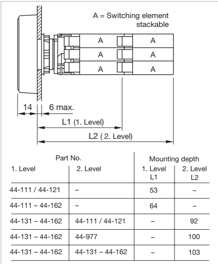
Dimensions [mm]
