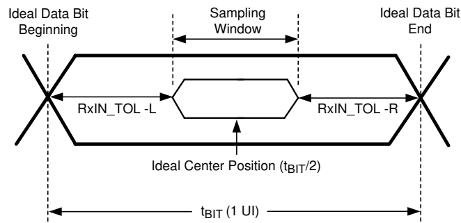
Figure 5-16. Deserializer Setup and Hold Times and PTO Spread, PTOSEL = L
