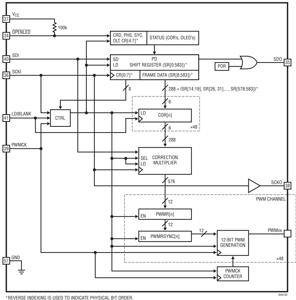
Figure 1. Block Diagram
