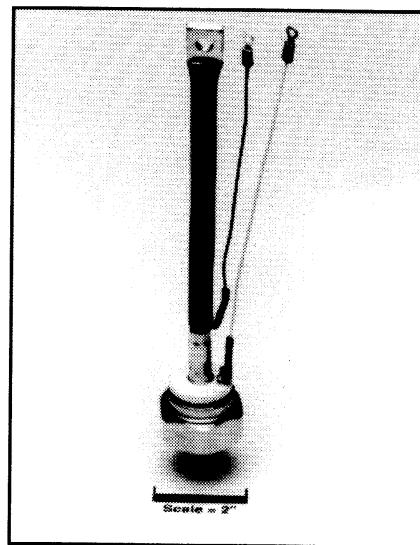
T700 Phase Control SCR 300-350 Amperes, 2400 Volts
