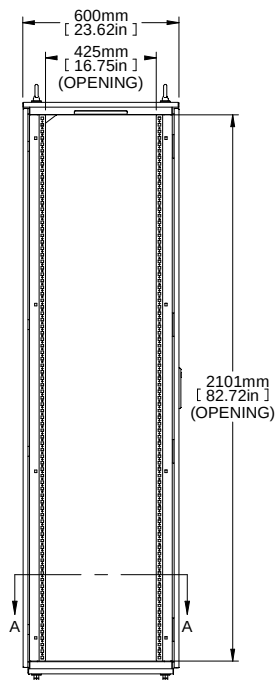
L.S. VIEW
