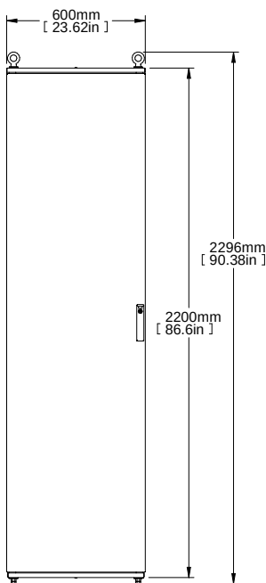
FRONT VIEW
