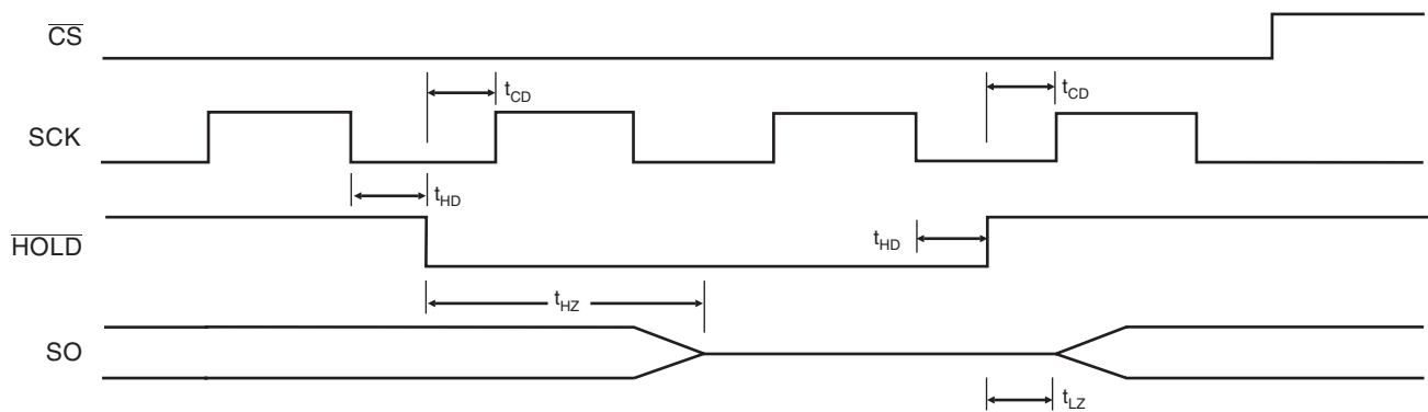
Figure 10. \overline{HOLD} Timing
