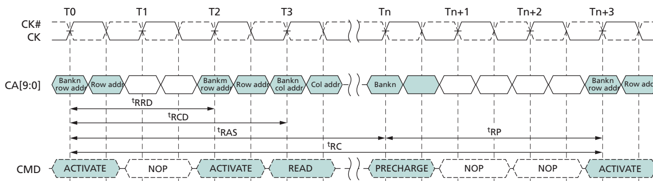
Figure 27: ACTIVATE Command
