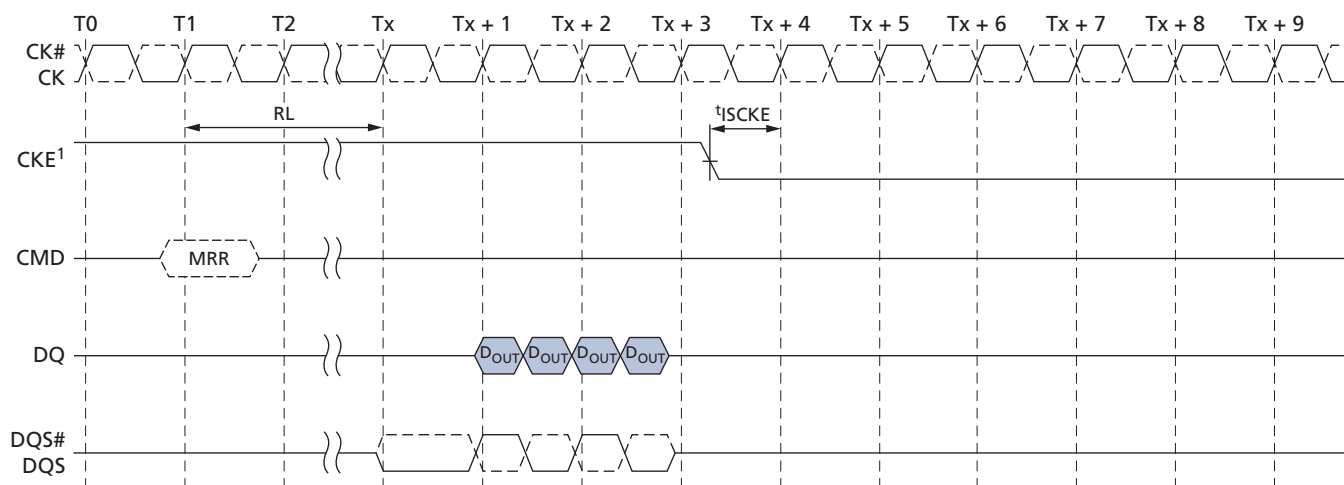
Figure 78: MRR Command to Power-Down Entry
