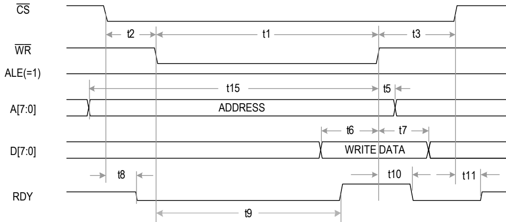
Figure - 26. Non-Multiplexed Intel Mode Write Timing
