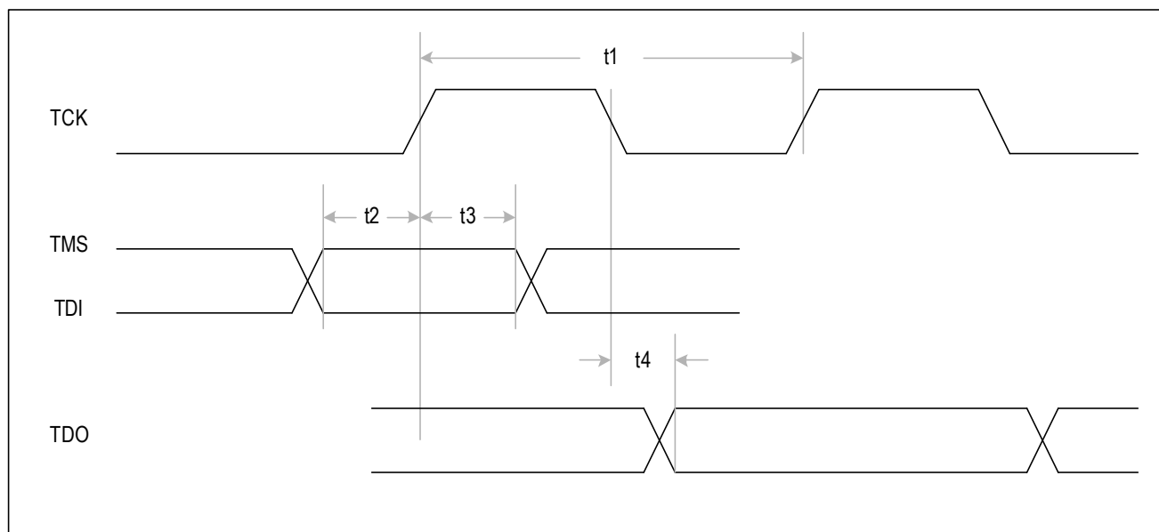
Figure - 23. JTAG Interface Timing
