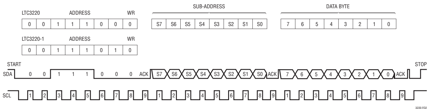
Figure 2. Bit Assignments
