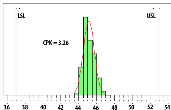
Figure 1. Idd1 distribution ; LSL=37mA , USL=53mA
