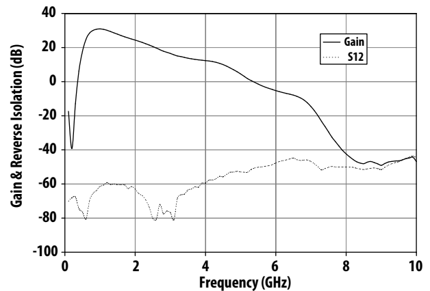
Figure 15. Gain & S12 vs. Frequency
