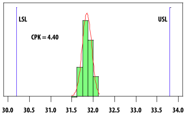
Figure 3. Gain distribution ; LSL=30.2dB , USL=33.8dB
