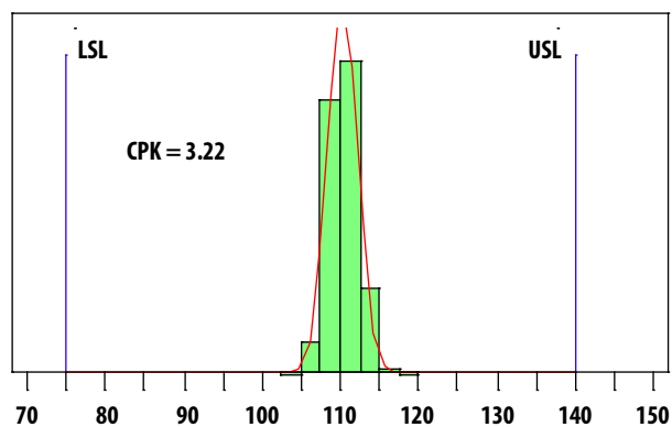
Figure 2. Idd2 distribution ; LSL=75mA , USL=140mA
