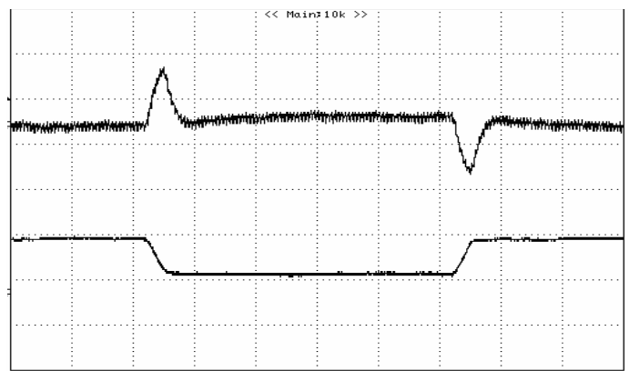
Figure 26: Typical transient response to step load change at 5A/\mu S from 25% to 75% of I_o , max at 12Vin, 5V out ( C_{out} = 1\mu F ceramic, 10\mu F tantalum) Top: 100mV/div, 50uS/div, Bottom: 20A/div, 50uS/div
