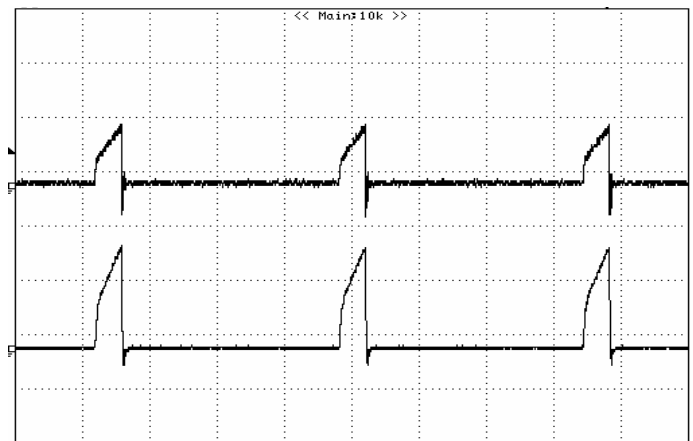
Figure 26: Typical transient response to step load change at 5A/\mu S from 25% to 75% of I_o , max at 12Vin, 5V out ( C_{out} = 1\mu F ceramic, 10\mu F tantalum) Top: 100mV/div, 50uS/div, Bottom: 20A/div, 50uS/div
