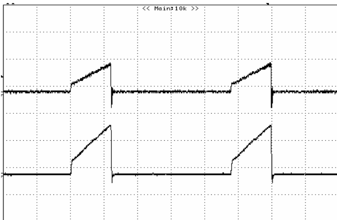
Figure 25: Typical transient response to step load change at 5A/\mu S from 25% to 75% of I_o , max at 12Vin, 3.3V out ( C_{out} = 1\mu F ceramic, 10\mu F tantalum) Top: 100mV/div, 50uS/div, Bottom: 20A/div, 50uS/div
