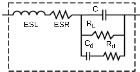
Figure 3 The Real Capacitor
