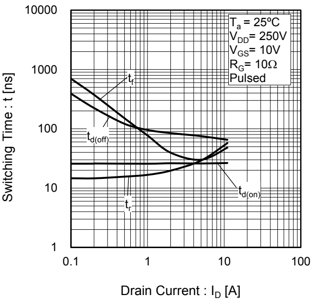
Fig.20 Switching Characteristics
