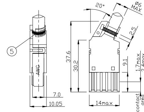
OVERALL VIEW
