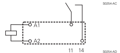
Pinning 5 mm
