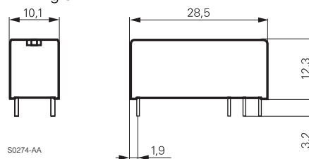
Pinning 3.2 mm
