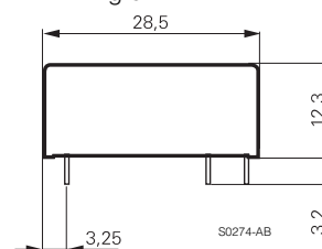
Pinning 5 mm
