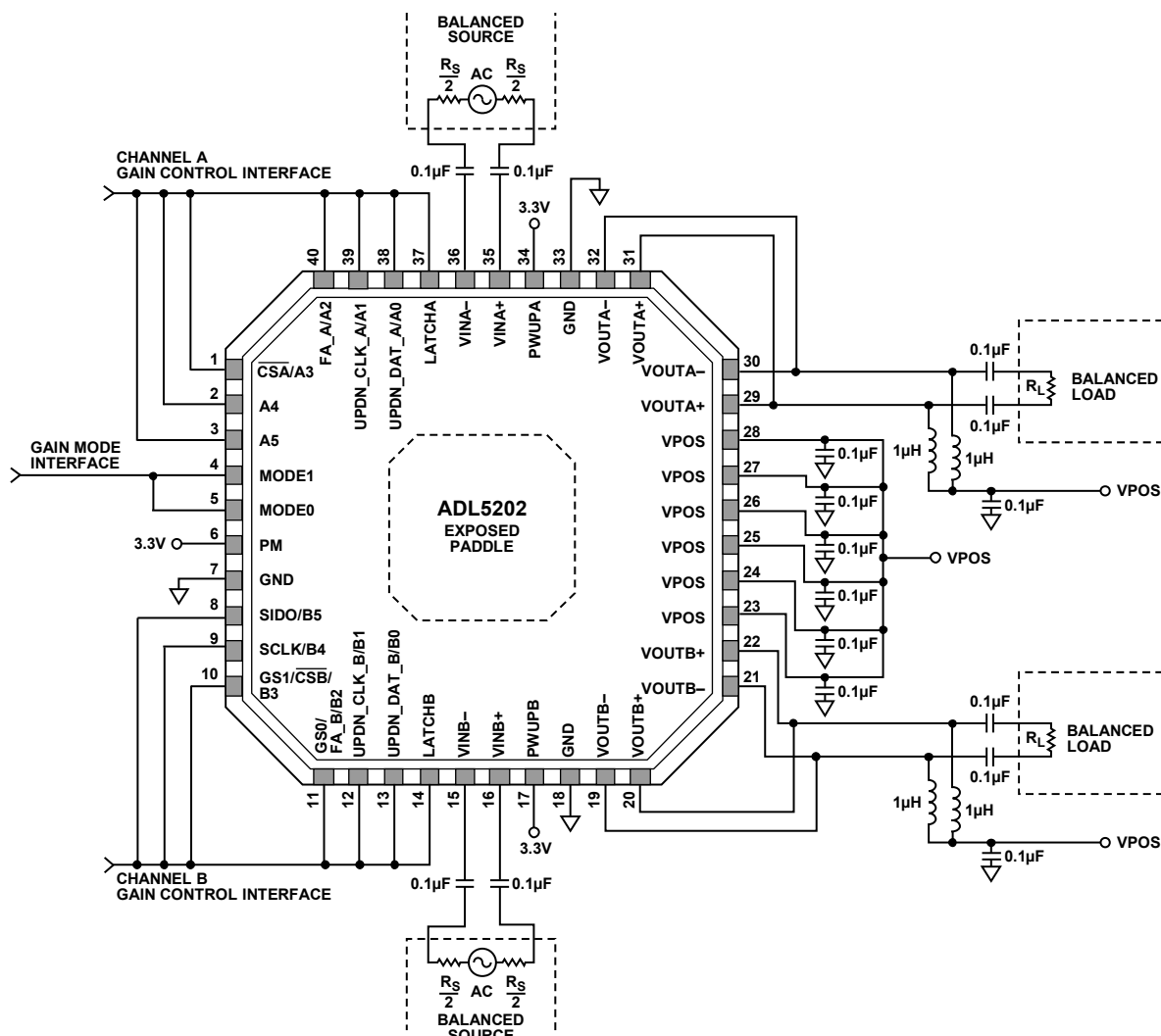
Figure 54. Basic Connections
