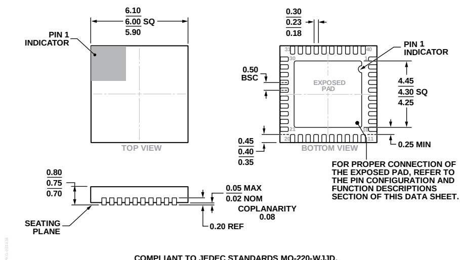
Figure 66. 40-Lead Lead Frame Chip Scale Package [LFCSP_WQ] 6 mm × 6 mm Body, Very Very Thin Quad (CP-40-10) Dimensions shown in millimeters
