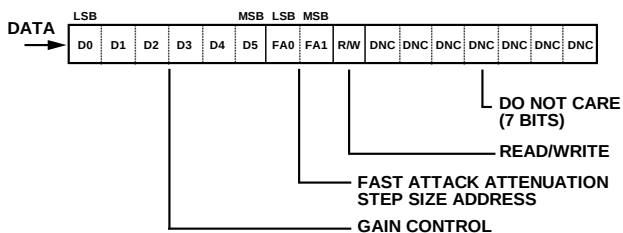
Figure 50. 16-Bit SPI Register
