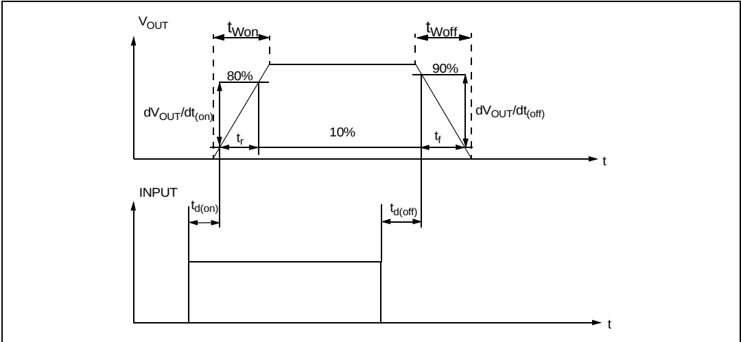
Figure 8. Switching characteristics
