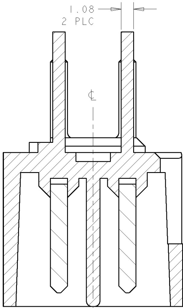
SECTION B-B
