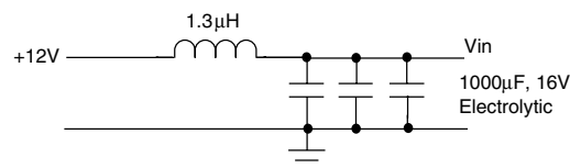
Figure 5. Input Filter
