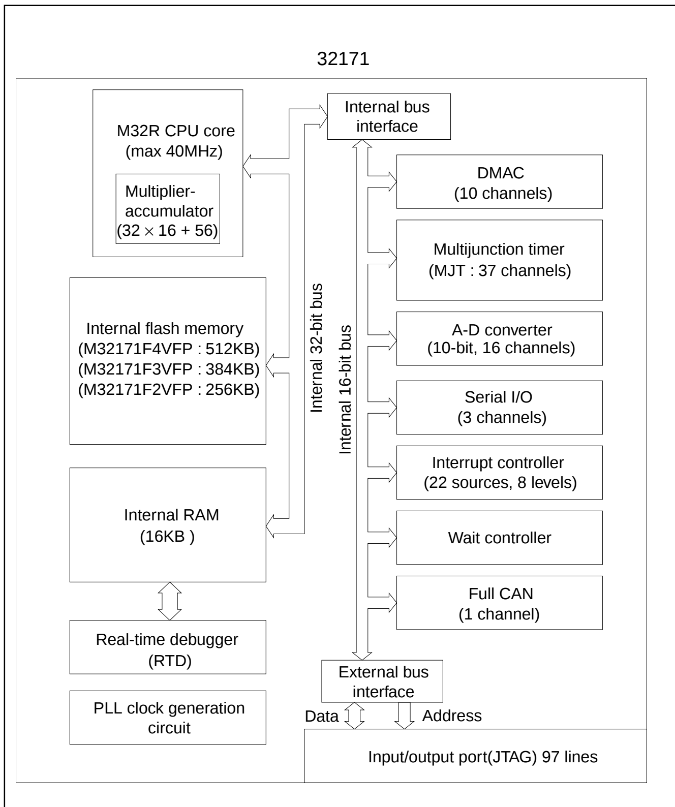
Figure 2 Block diagram
