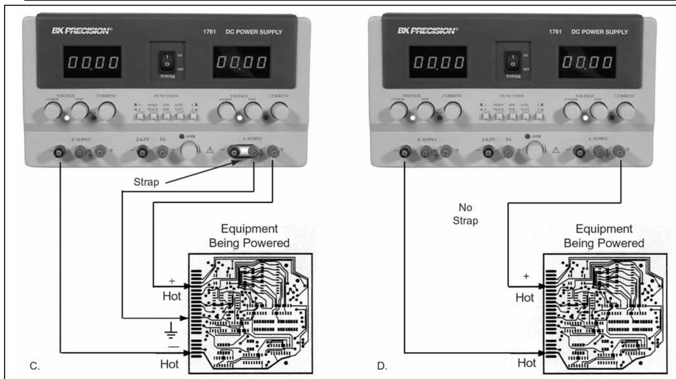
Fig. 8. Series Tracking (0-to-60V) Operation Grounding Possibilities
