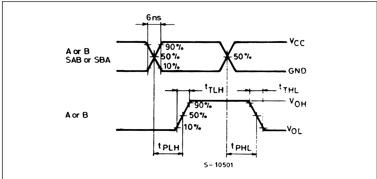
WAVEFORM 1 : PROPAGATION DELAY TIME ( f=1\text{MHz} ; 50% duty cycle)
