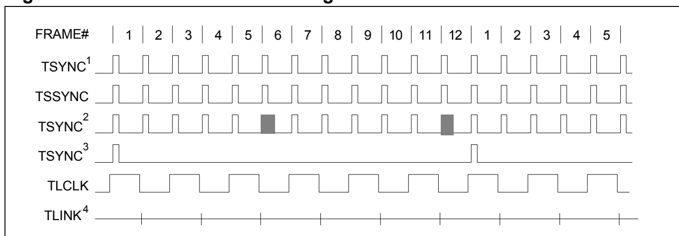
Figure 31-6. Transmit-Side D4 Timing
