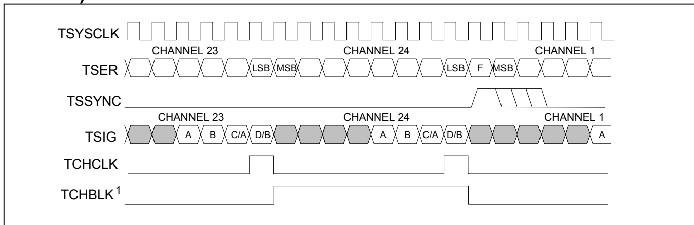
Figure 31-9. Transmit-Side 1.544MHz Boundary Timing (with Elastic Store Enabled)
