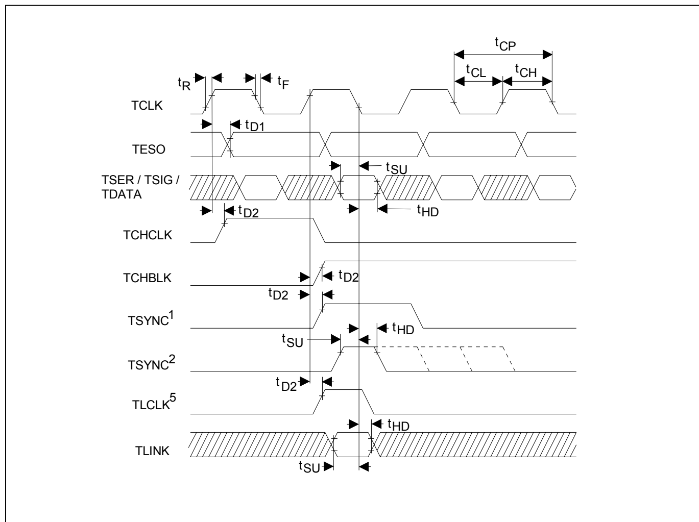
Figure 33-11. Transmit-Side Timing
