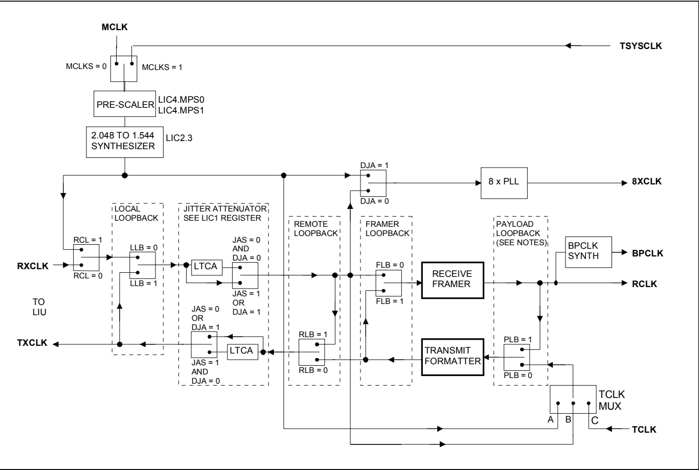
Figure 6-1. Clock Map
