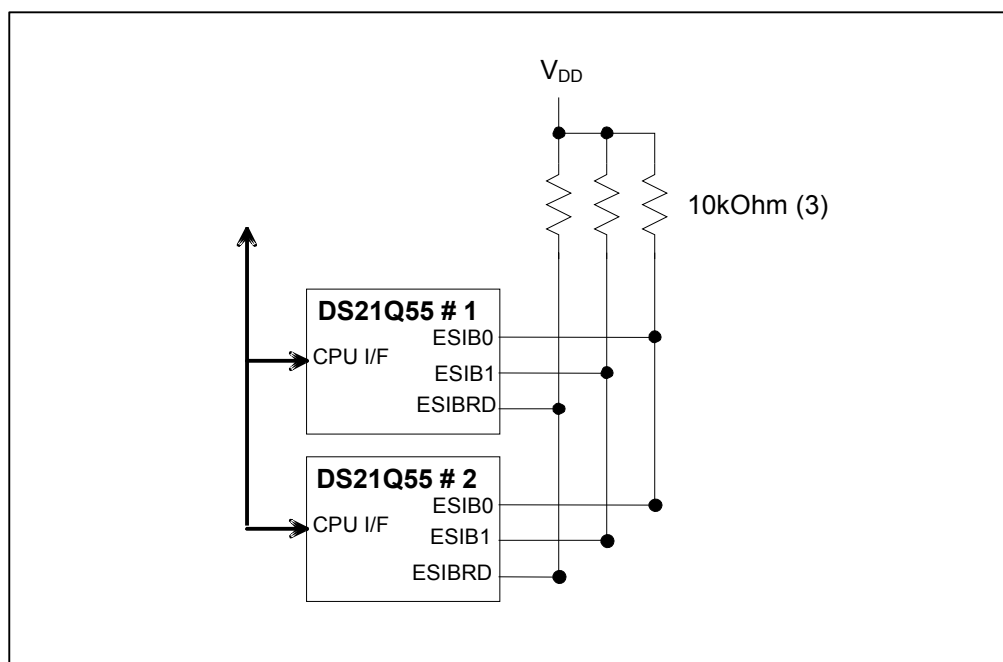
Figure 27-1. ESIB Group of Two DS21Q55s
