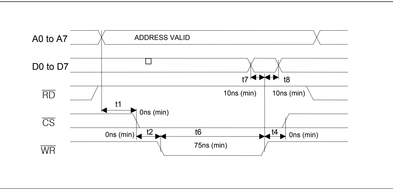
Figure 33-5. Intel Bus Write Timing (BTS = 0/MUX = 0)
