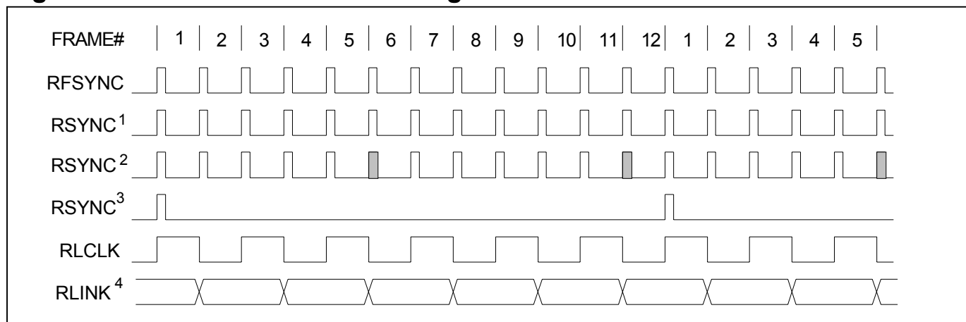
Figure 31-1. Receive-Side D4 Timing
