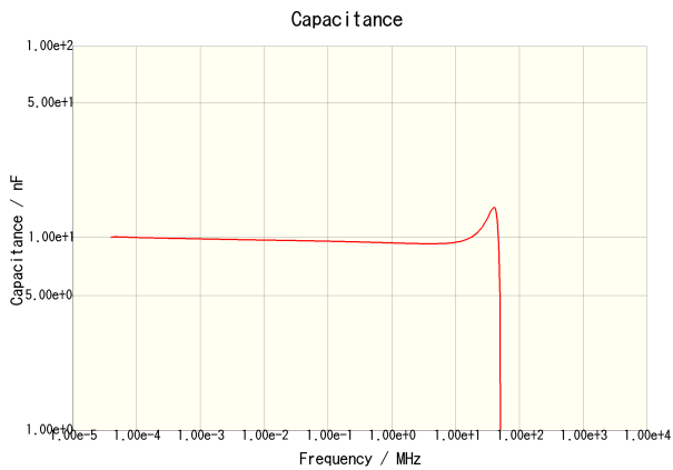
CKCL44X7R1E103M085AA
