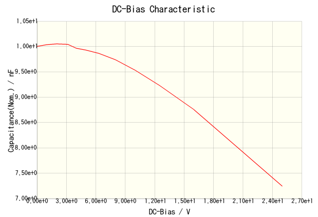
CKCL44X7R1E103M085AA
