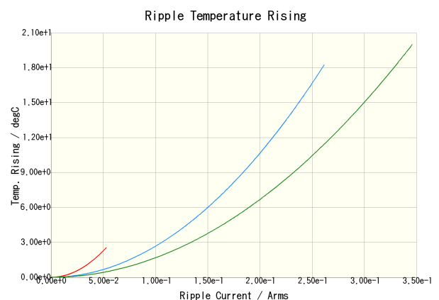
CKCL44X7R1E103M085AA(100kHz) CKCL44X7R1E103M085AA(500kHz) CKCL44X7R1E103M085AA(1MHz)
