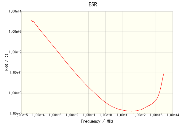
CKCL44X7R1E103M085AA
