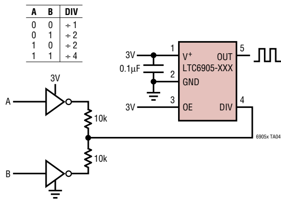
Driving the DIV Pin Without Three-State Buffers
