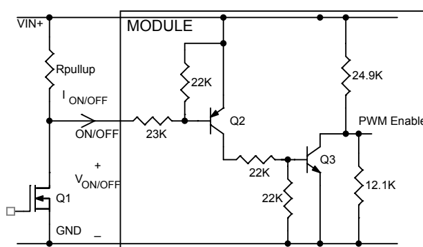
Circuit configuration for using positive On/Off logic
