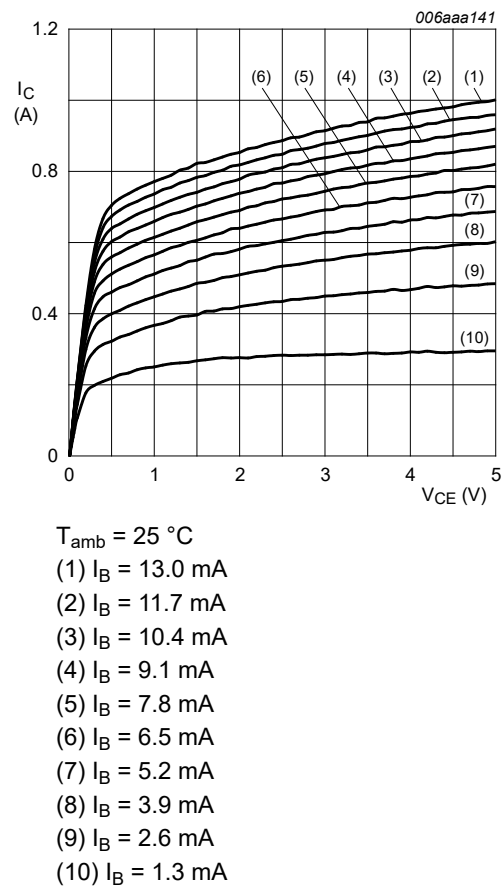
Fig. 11. BC817-25: Collector current as a function of collector-emitter voltage; typical values
