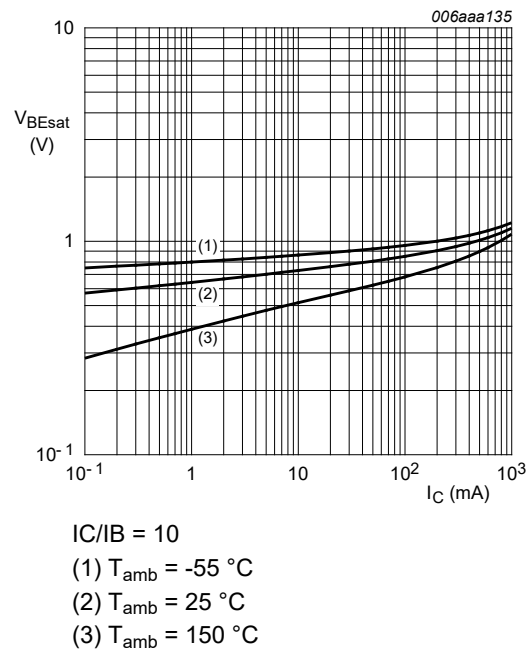
Fig. 9. BC817-25: Base-emitter saturation voltage as a function of collector current; typical values
