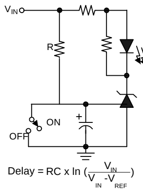
Fig. 5 Delay Timer
