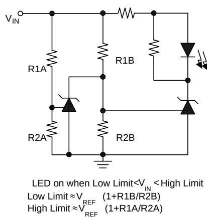
Fig. 4 Voltage Monitor
