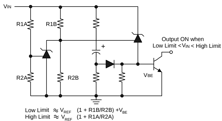
Fig. 10 Over-Voltage / Under-Voltage Protection Circuit
