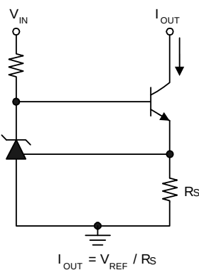
Fig. 7 Constant-Current Sink
