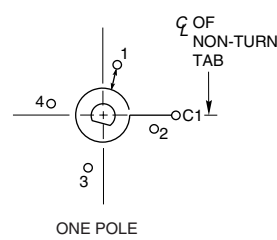
Series 09 90° Angle of Throw
