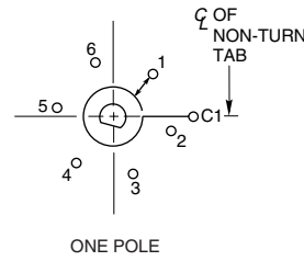
Series 09 60° Angle of Throw
