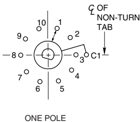
Series 08 36° Angle of Throw
