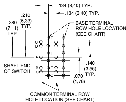
30°, 60° and 90° Angle of Throw
