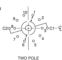
Series 09 90° Angle of Throw
