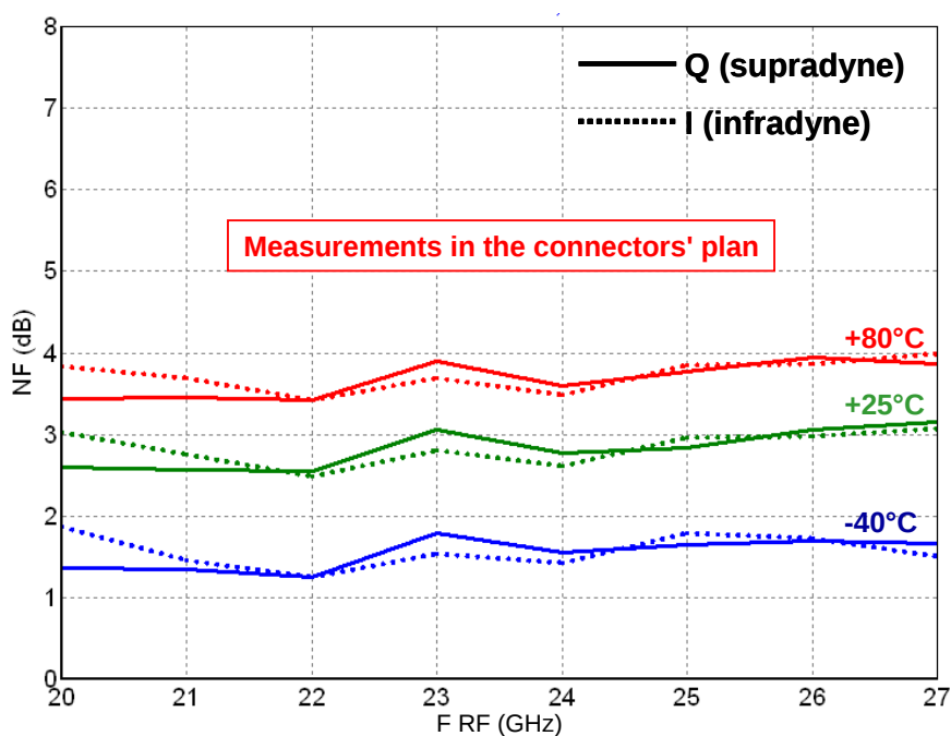
Noise figure channel I & Q @ -40, +25, +80°C
