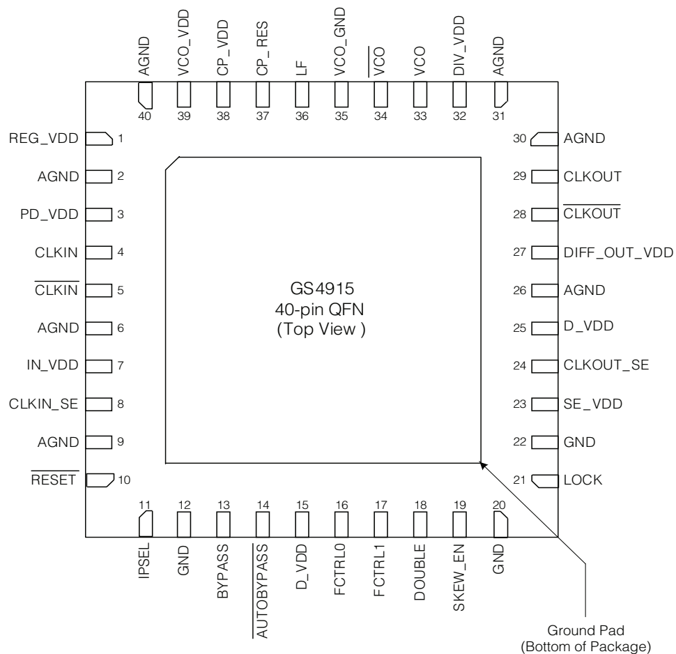
Figure 1-1: 40-Pin QFN
