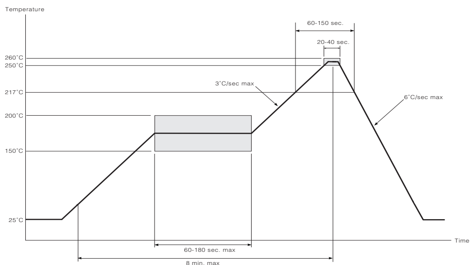
Figure 2-2: Maximum Pb-Free Solder Reflow Profile (Preferred)
