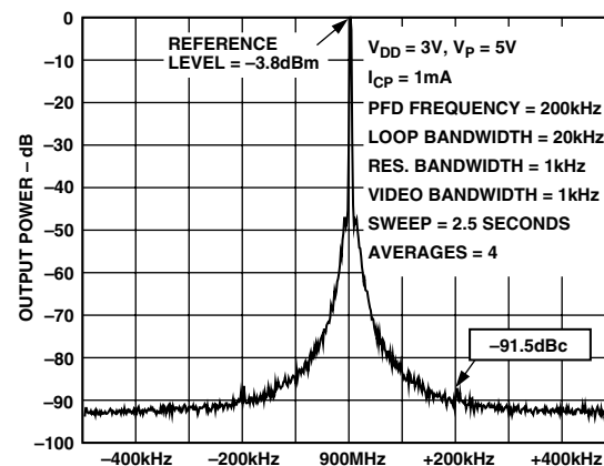
TPC 6. ADF4118 Reference Spurs (900 MHz, 200 kHz, 20 kHz)
