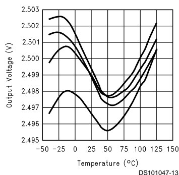
Typical Temperature Drift
