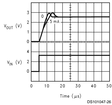
Start-Up Response
