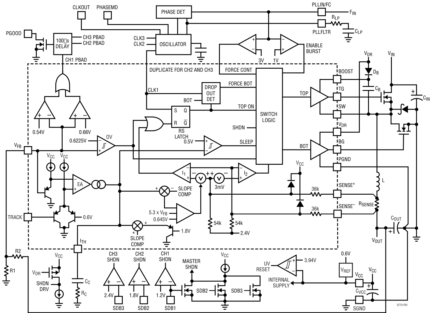
Figure 1. Functional Diagram
