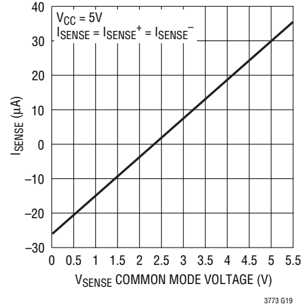
SENSE Pin Input Current vs SENSE Common Mode Voltage
