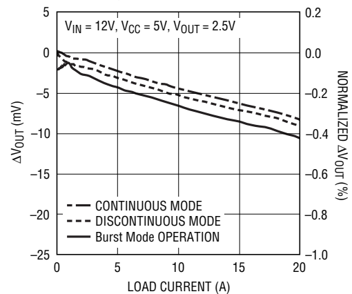
Load Regulation
