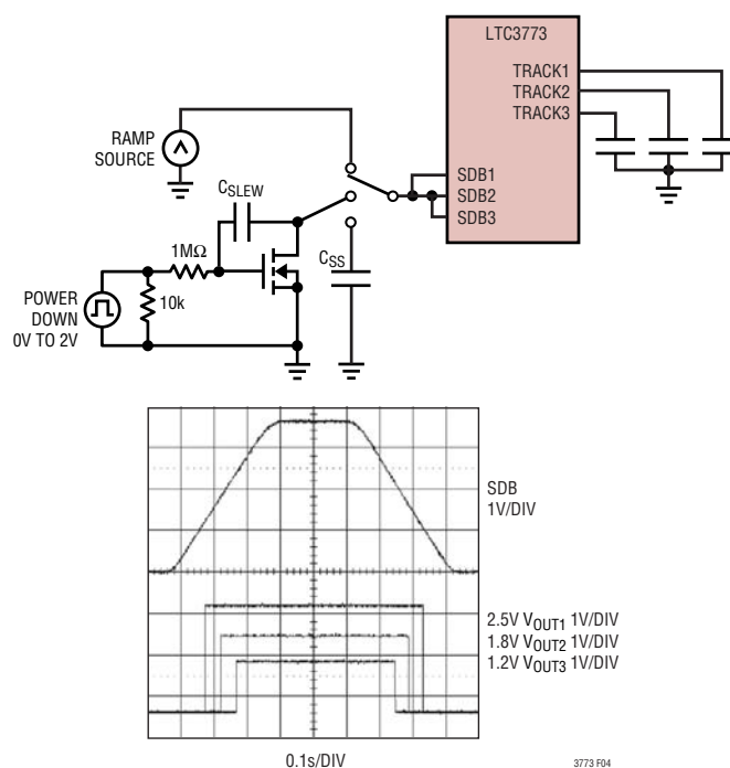
Figure 4. Sequential Power Up/Down
