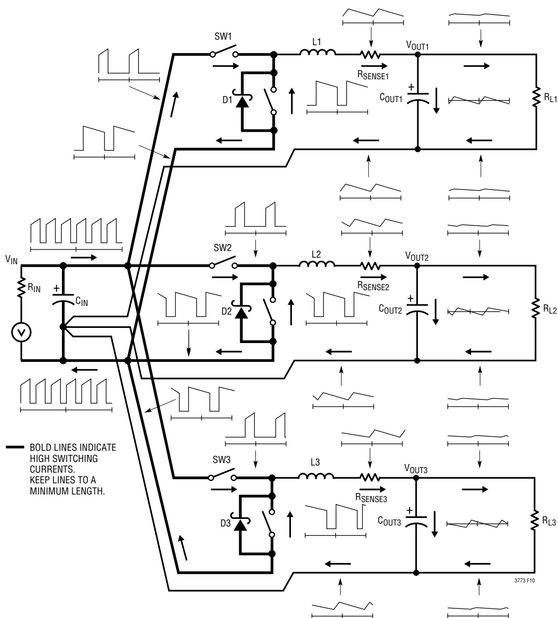
Figure 10. Branch Current Waveforms
