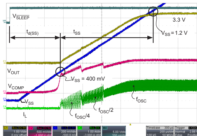
Figure 4: Normal Startup to V_{\text{OUT}} = 3.3 \text{ V} , I_{\text{OUT}} = 1.6 \text{ A} , SLEEP Transitions High
