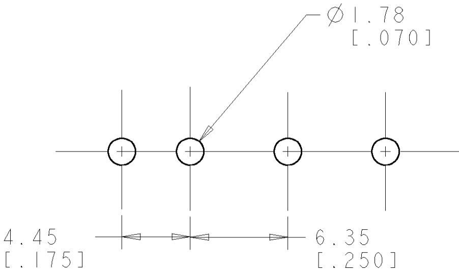
RECOMMENDED MOUNTING HOLE PATTERN FOR 1.57 [.062] THICK P.C. BOARD
